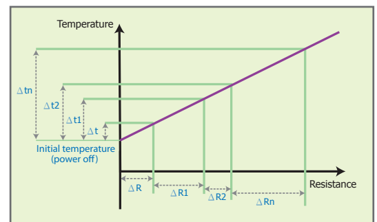
Temperature Correction
