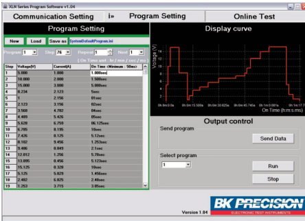
Generate, save, and load program lists. View output characteristic curves and export data to a file.
