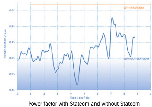
Power factor with Statcom and without Statcom
