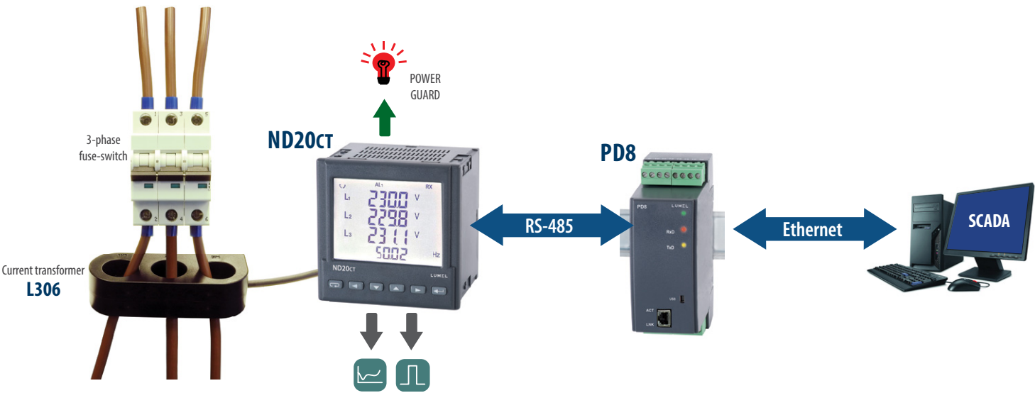
Measurements, monitoring, recording of network parameters and energy using a three-phase transformer with screw terminals.
