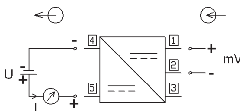
Voltage 0 .. 60 mV
