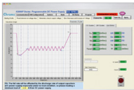
ISO 16750-2 4.5.3 Starting Profile
